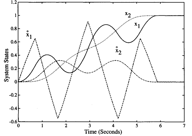
Fig. 5 Evolution of system states subject to robust time-optimal control.
