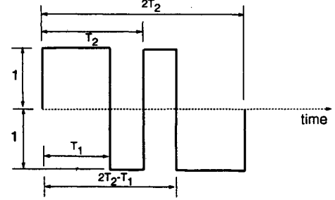
Fig. 2 Antisymmetric control profile for a spring-mass system.
