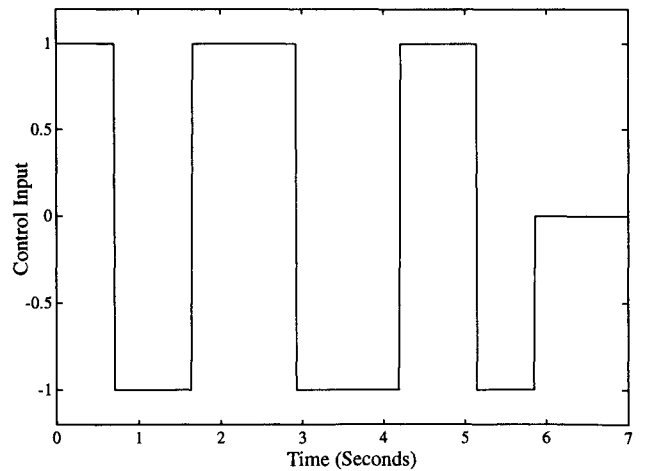
Fig. 6 Robust time-optimal control profile for a spring-mass system.
