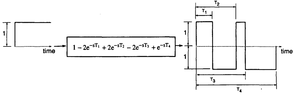
Fig. 1 Time-delay filter.
